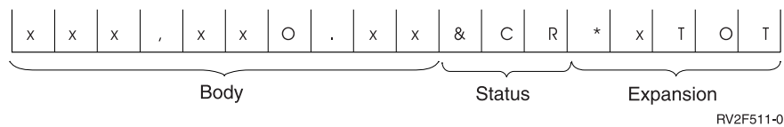
Figure 18. Three parts of an edit word
